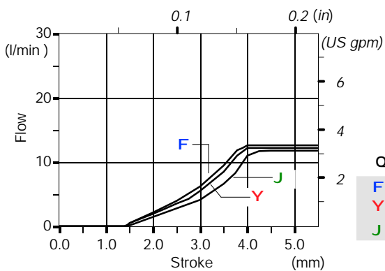
Spool metering P to A
