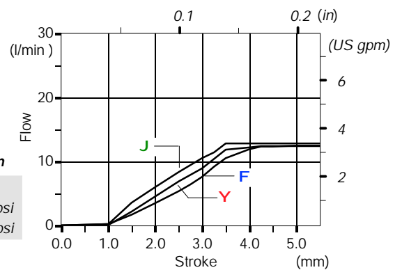
Spool metering A to T
