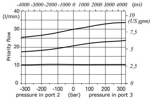
Flow pressure diagram from port 2 ⇒ port 3
