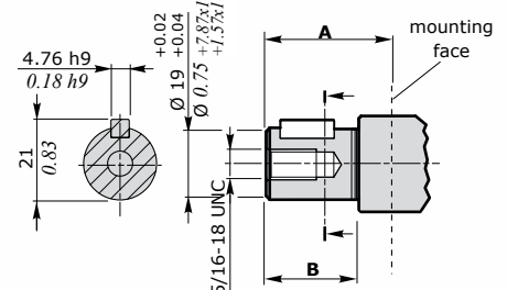
Shaft dimensions
