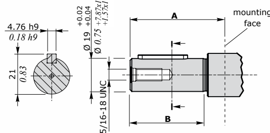
Shaft dimensions
