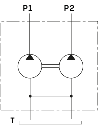
Hydraulic circuit
