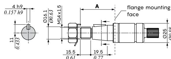
Shaft dimension
