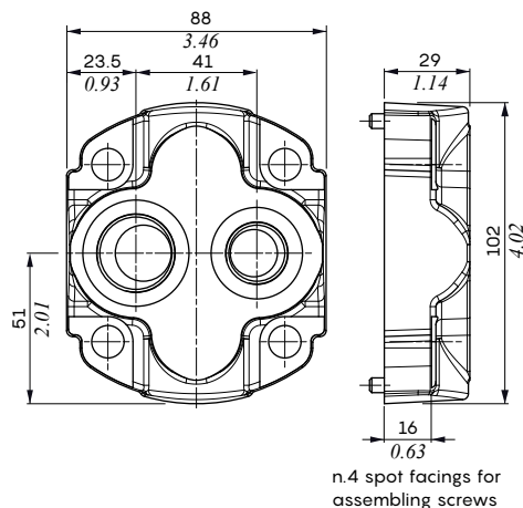
Connection position 1/3/4
