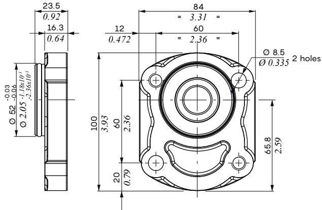
E52CX configuration
