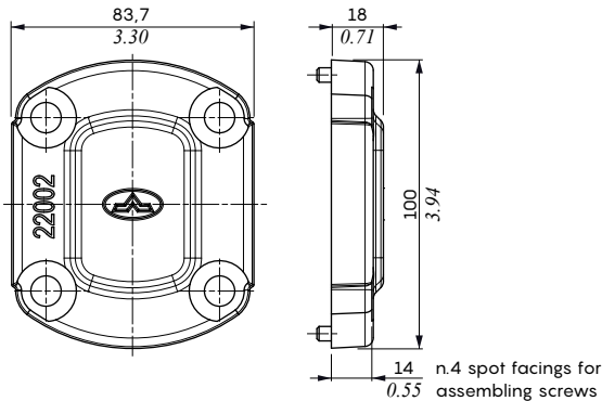
Connection position 0
