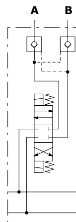
QBP type example (with spool 1)
