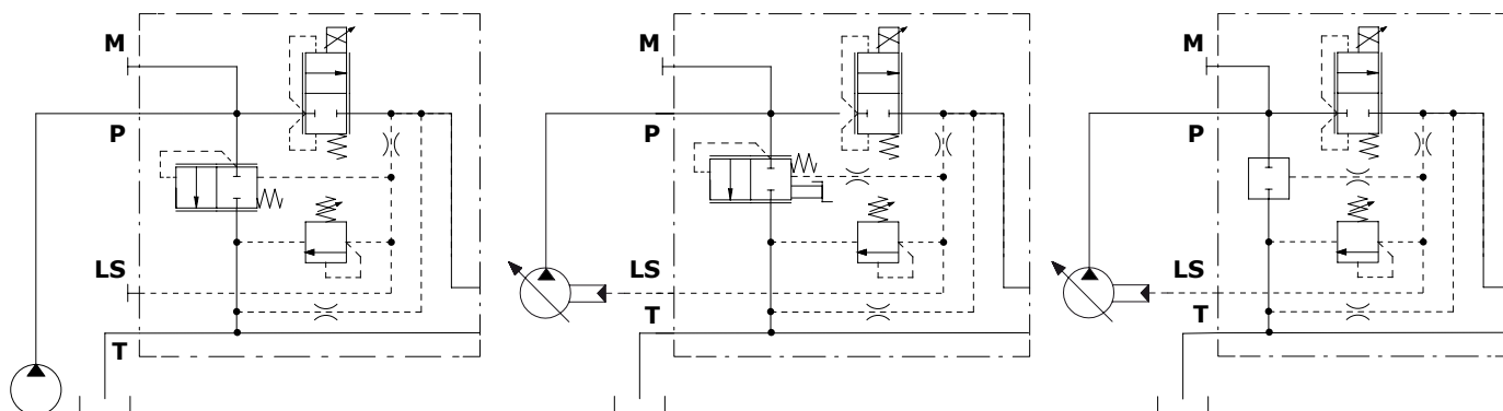
AN6 type for Open Center circuit
