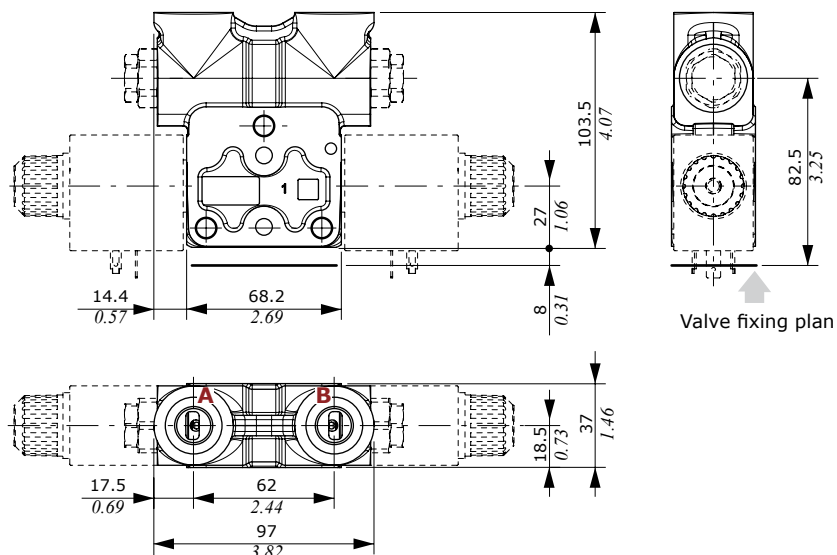
QBP - QBPE types with check valve arrangement
