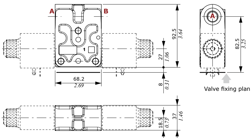
QL - QBPL types with or without check valves arrangement
