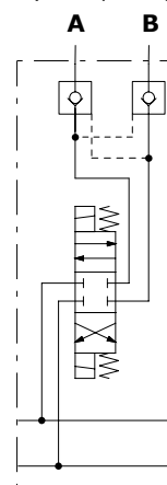
QBPL type example (with spool 1)
