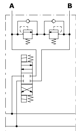
PFL type example (with spool 1)
