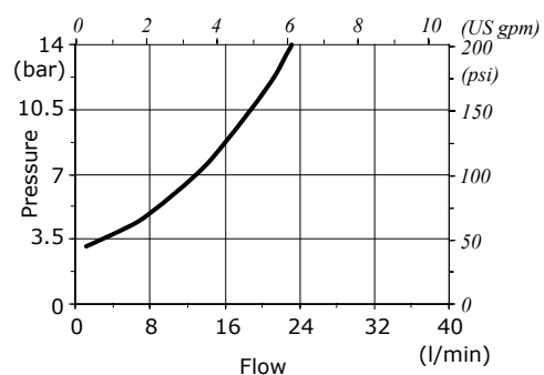
A1(B1) \Rightarrow A2(B2) pressure drops (with series circuit)
