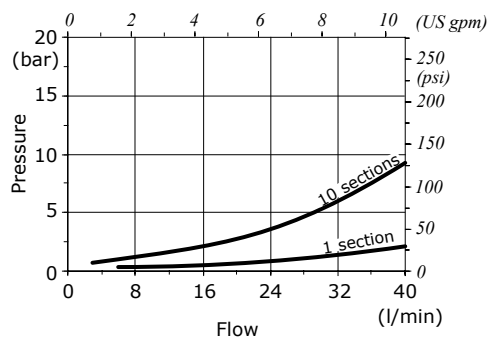
A(B) \Rightarrow T pressure drops
