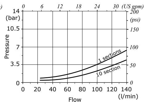
A(B)⇒T pressure drops
