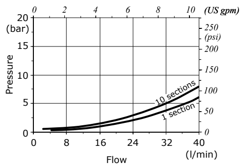
A1(B1) \Rightarrow A2(B2) pressure drops (with series circuit)
