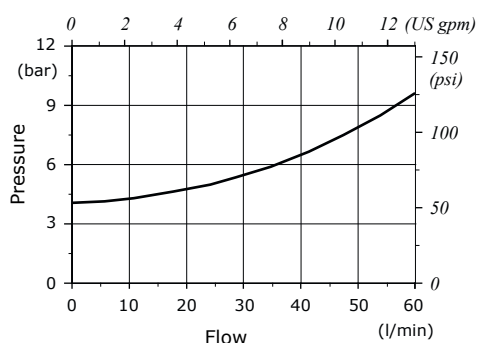
Pressure drops
