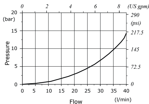
Pressure drops
