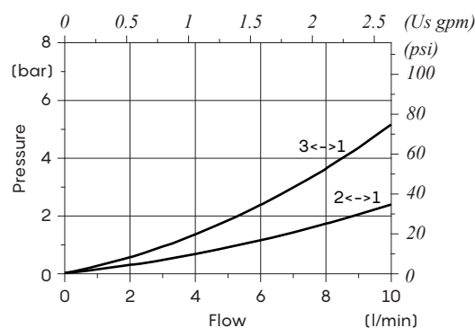
Pressure drop vs. flow Spool 5
