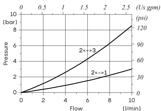
Pressure drop vs. flow Spool 6
