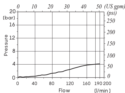
LA16QA pressure drop (fully open)
