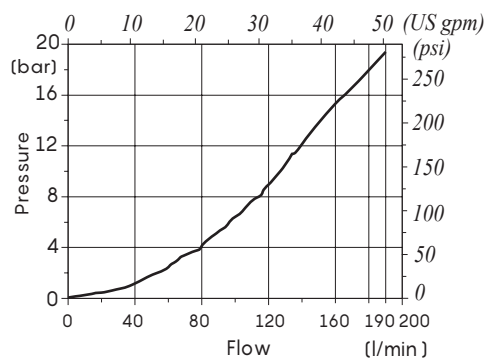
LC16QA pressure drop (fully open)
