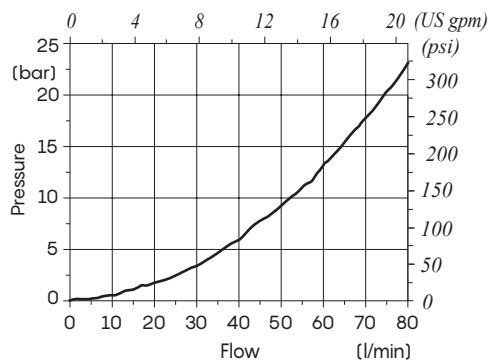
LC10QA pressure drop (fully open)
